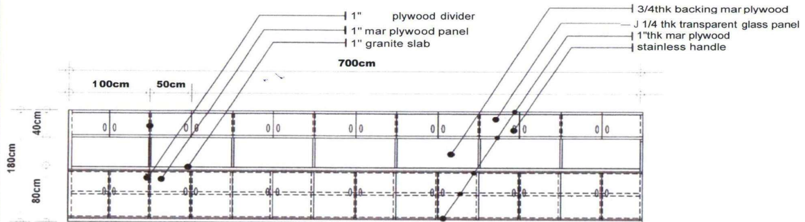
FRONT VIEW
